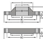
Class 75 Industry Std Weldneck
