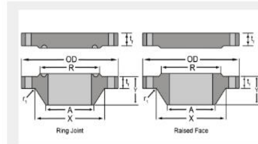
ASME B16.47 Series A Class 300
