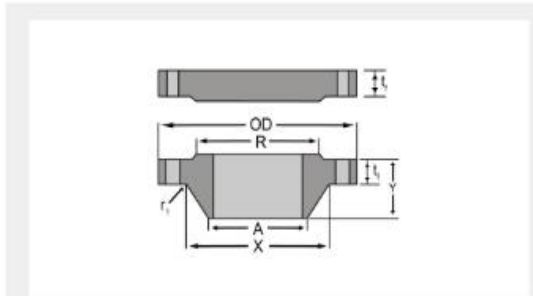
ASME B16.47 Series A Class 150
