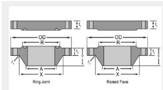
ASME B16.47 Series A Class 400
