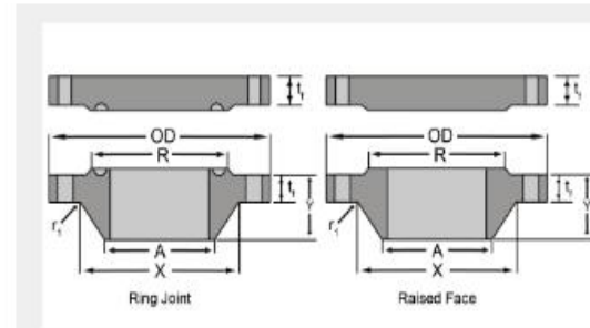
ASME B16.47 Series A Class 600
